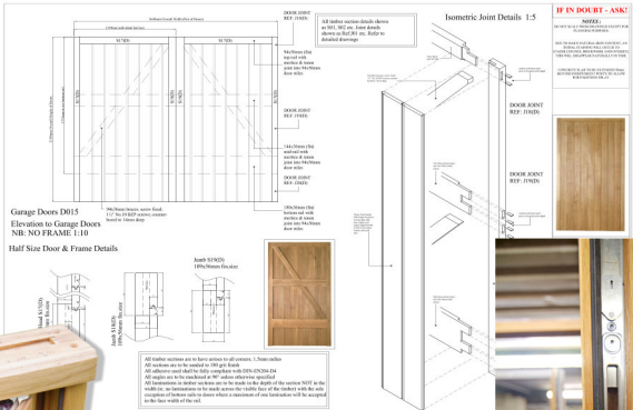
Oak Joinery with Friction Hinges & Multi Locking
